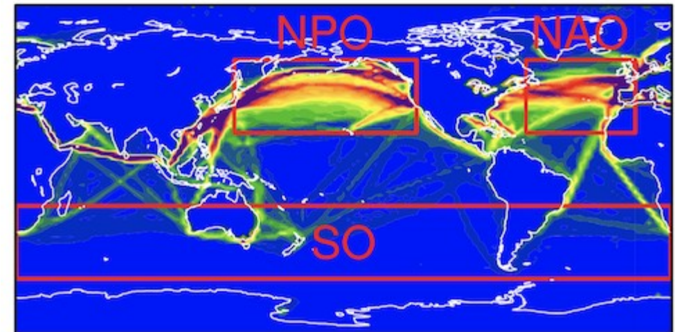
(a) Shipping SO 2
